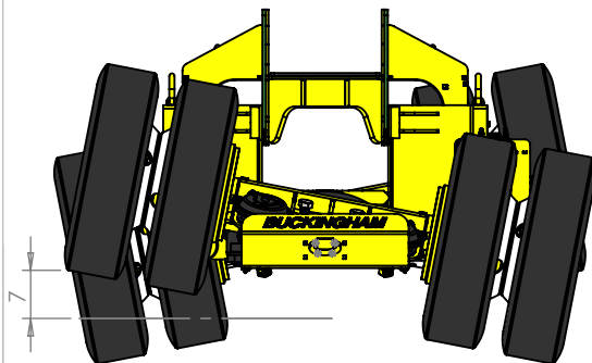
OSCILLATING AXLES
